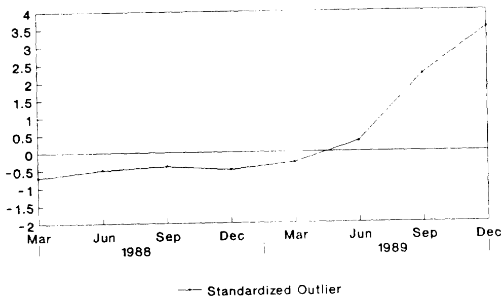
Figure 4. SDOC Control Chart, Georgia, December 1989
