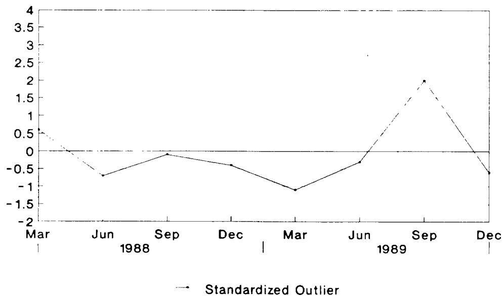
Figure 2. SDOC Control Chart U.S. level, December 1989
